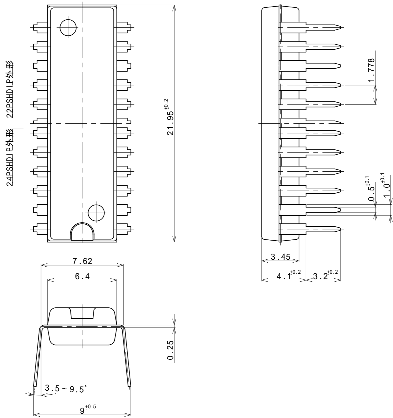
SHDIP22/24P(300mil)
